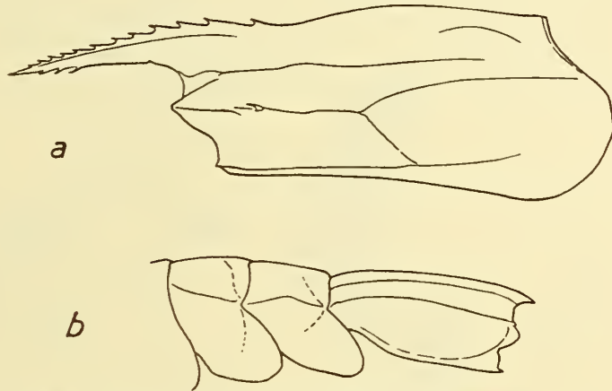
TEXT-FIG. 10.— Funchalia (Pelagopenæus) balboæ (Faxon). a , Carapace, \times 4.7 . b , Three posterior abdominal segments, \times 4.7 .
